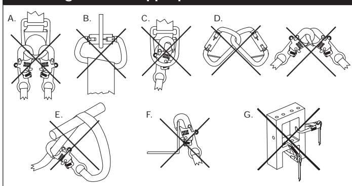
Figure 5 - Inappropriate Connections
