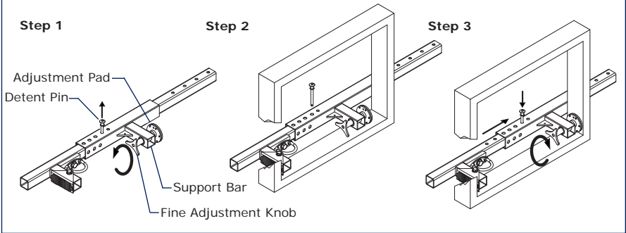
FIGURE 6 - INSTALLATION
